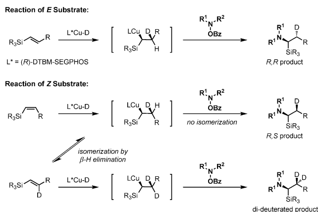
Scheme 7. Possible reaction pathways.
