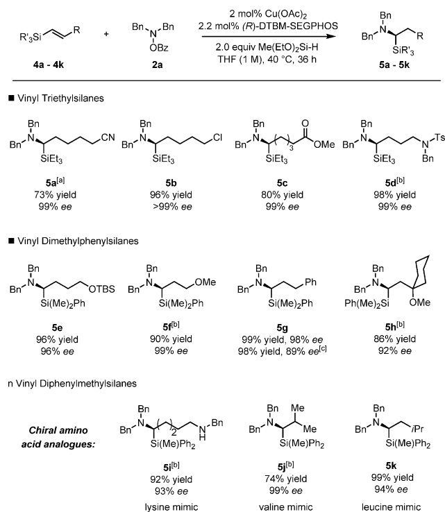
Scheme 5. Hydroamination of ( E )-vinylsilanes. Reaction conditions: 4a–4k (1 mmol), 2a (1.2 mmol), Cu(OAc) 2 (0.02 mmol), (R)-DTBM-SEGPPOS (0.022 mmol), THF (1 mL), 40 °C, 36 h. Yields are of isolated products (average of two runs). [a] 16 h reaction time. [b] Cu(OAc) 2 (0.04 mmol), (R)-DTBM-SEGPPOS (0.044 mmol), THF (1 mL, 1 M). [c] From ( Z )- 4g . TBS = tert -butyldimethylsilyl, Ts = p -toluenesulfonyl.
