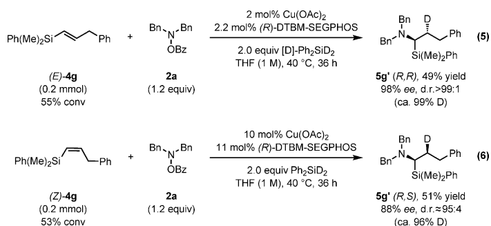
Scheme 8. Deuterium-labeling experiments.
