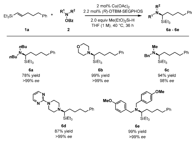
Scheme 6. Scope of O -benzoylhydroxylamine electrophiles. Reaction conditions: 1 (1 mmol), 2a (1.2 mmol), Cu(OAc) 2 (0.02 mmol), (R)-DTBM-SEGPPOS (0.022 mmol), THF (1 mL), 40 °C, 36 h. Yields are of isolated products (average of two runs).
