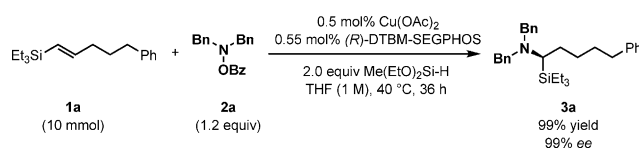
Scheme 9. Large-scale hydroamination reaction of ( E )-triethylsilylvinylsilane.
