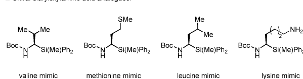
Scheme 1. Examples of silicon-containing peptidomimetics and amino acids. Boc = tert -butoxycarbonyl.
